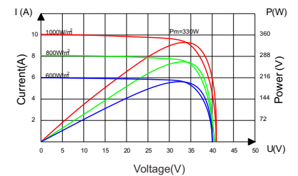
Current-Voltage&Power-Voltage Curve(330W)
