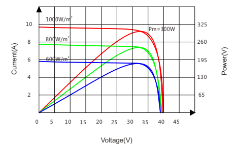
Current-Voltage&Power-Voltage Curve(300W)
