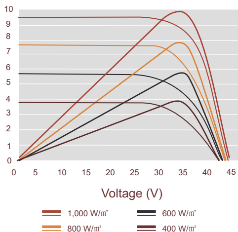
I-V Curves at Different Irradiances (335W) Test Temperature: 25°C
